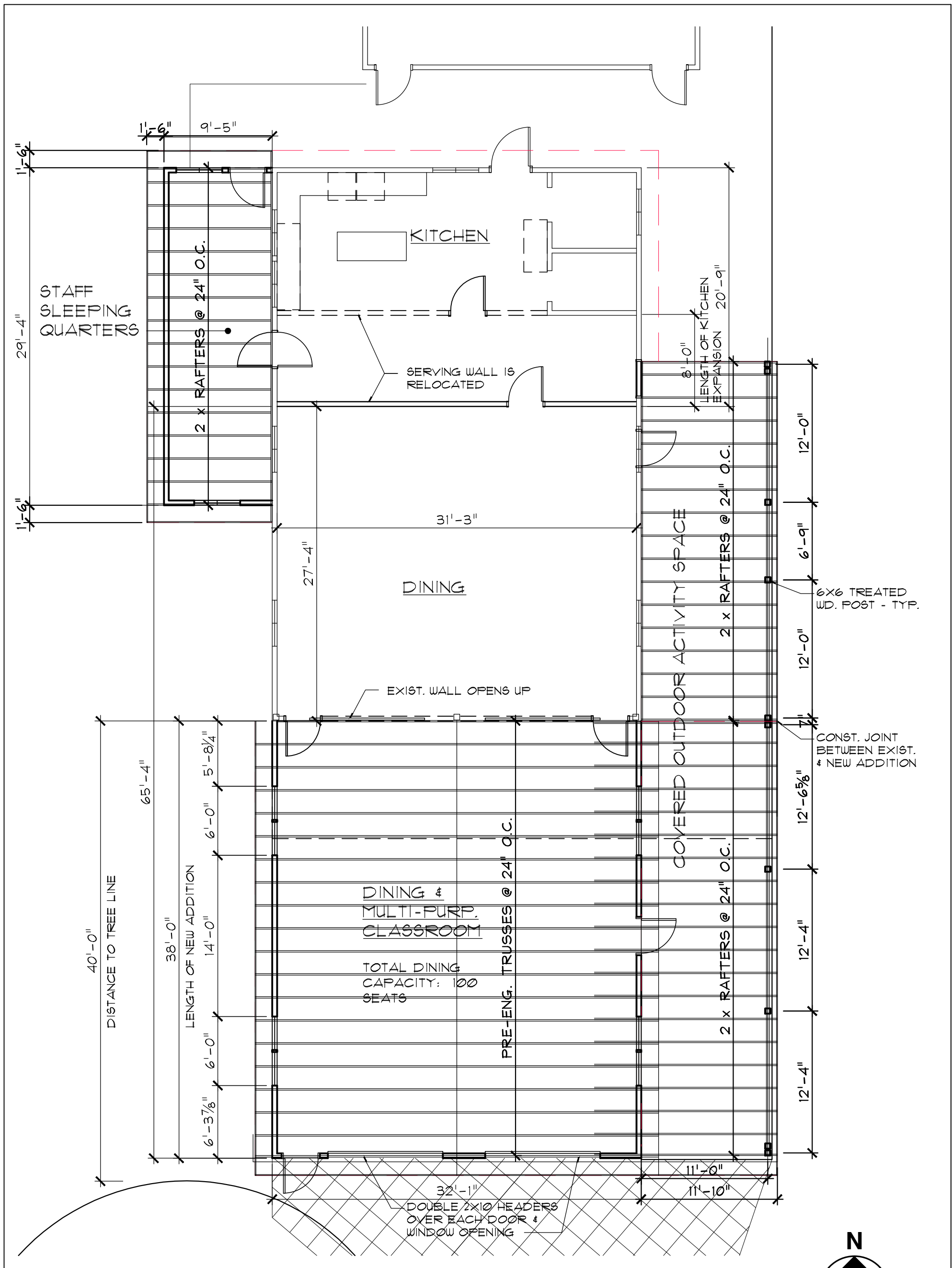
1 ROOF FRAMING PLAN A3 1/8" = 1'-0"
